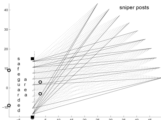
Fig. 5. The simulation of the system "2+4" for 1% measurement inaccuracies of directional measurements. Axes units are 1[m]. Dot lines shows successful evaluation of the sniper direction \hat{k} , and solid lines indicate cases of not convergent iterations.
