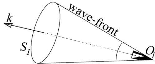
Fig. 1. The shock wave cone at the observation time t_1 when the supersonic bullet tip position is O_1 .
